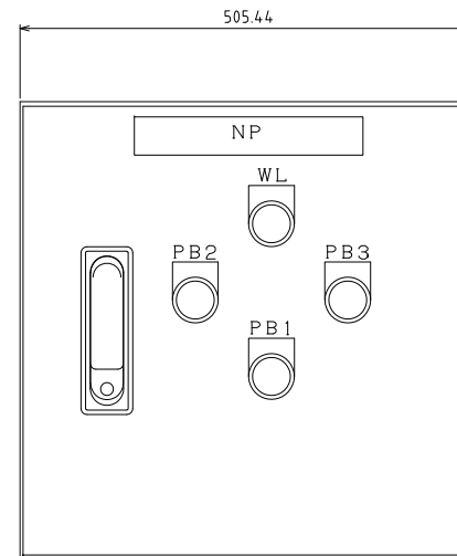
Control panel for Turn Table (Standard Motor wire length: 5m)
