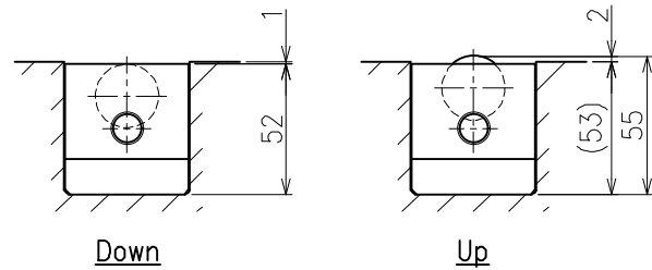
View-A
