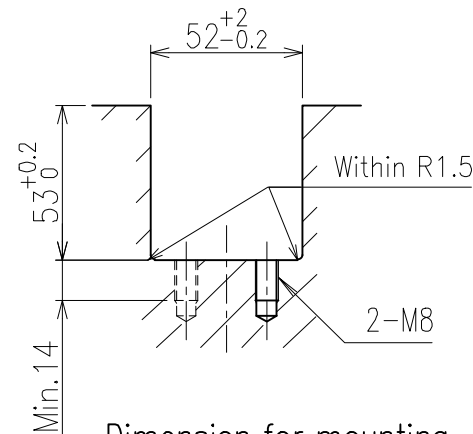
Dimension for mounting
