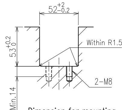
Dimension for mounting
