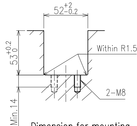
Dimension for mounting
